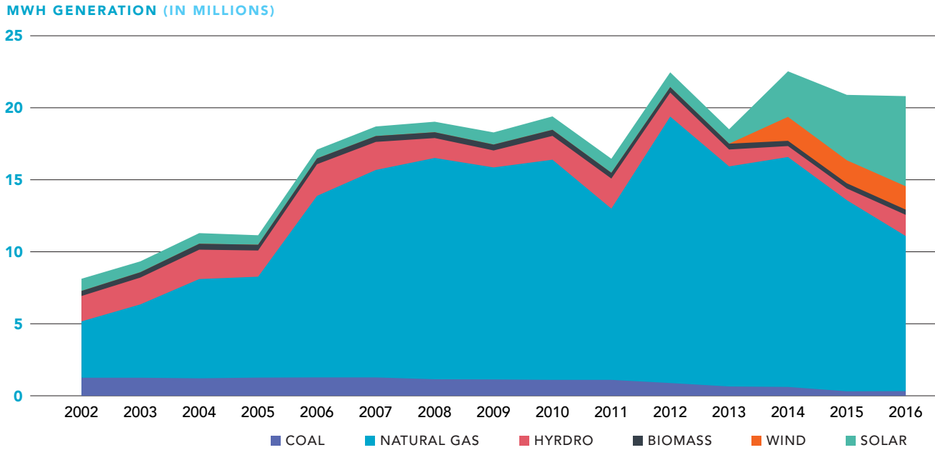
FIGURE 4 Electricity Generation by Source in the Inland Empire, 2002-2016
