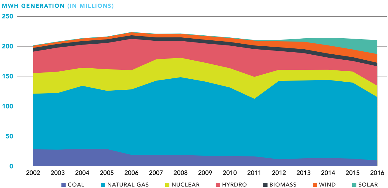
FIGURE 5 Electricity Generation by Source in California, 2002-2016
