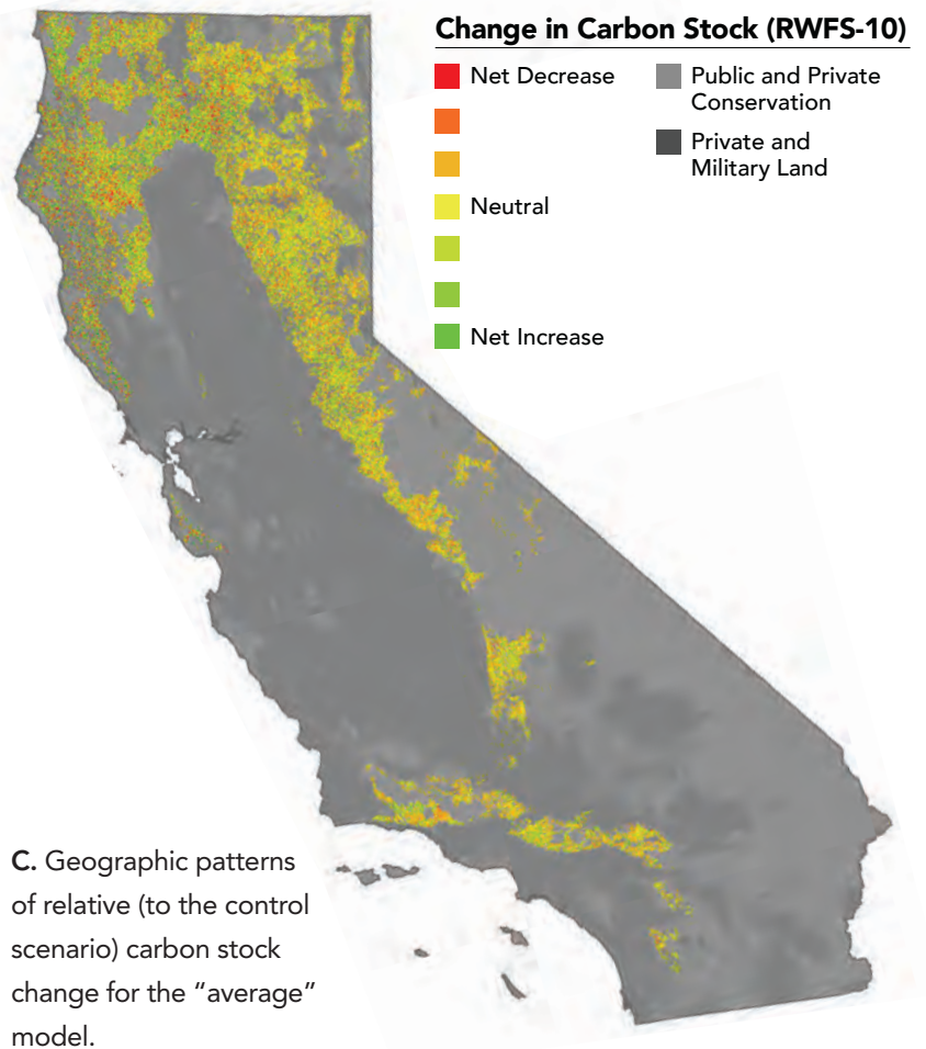
FIGURE 8 Overall Ecosystem Carbon Impact of Reduced Wildfire Severity (RWFS-10) Intervention, Assuming 10% High Severity Fire
