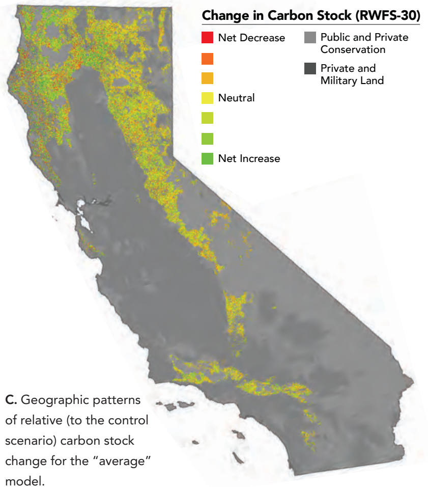
FIGURE 7 Overall Ecosystem Carbon Impact of Reduced Wildfire Severity (RWFS-30) Intervention, Assuming 30% High Severity Fire
